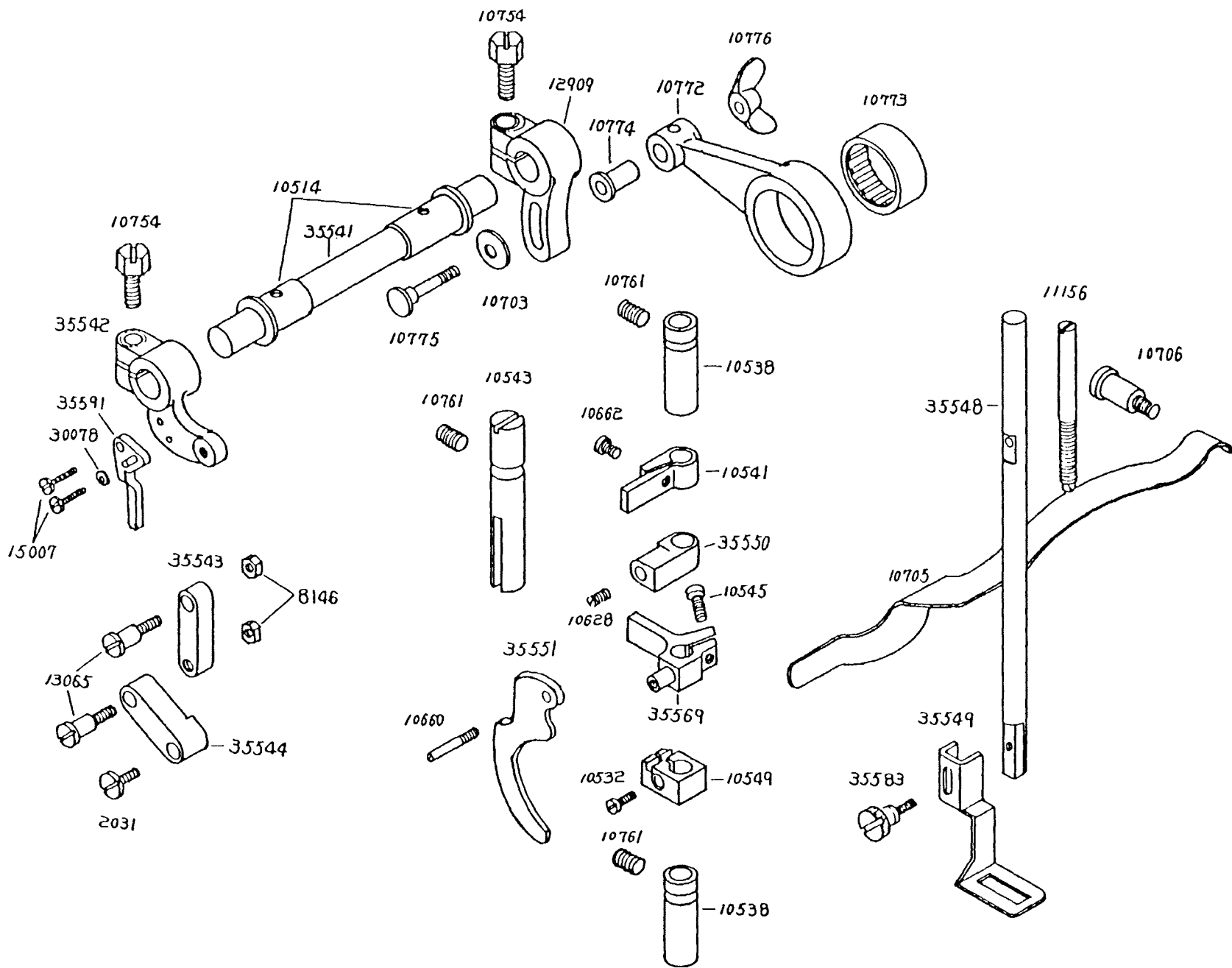
Fig. 7-31: Presser Bar & Components
