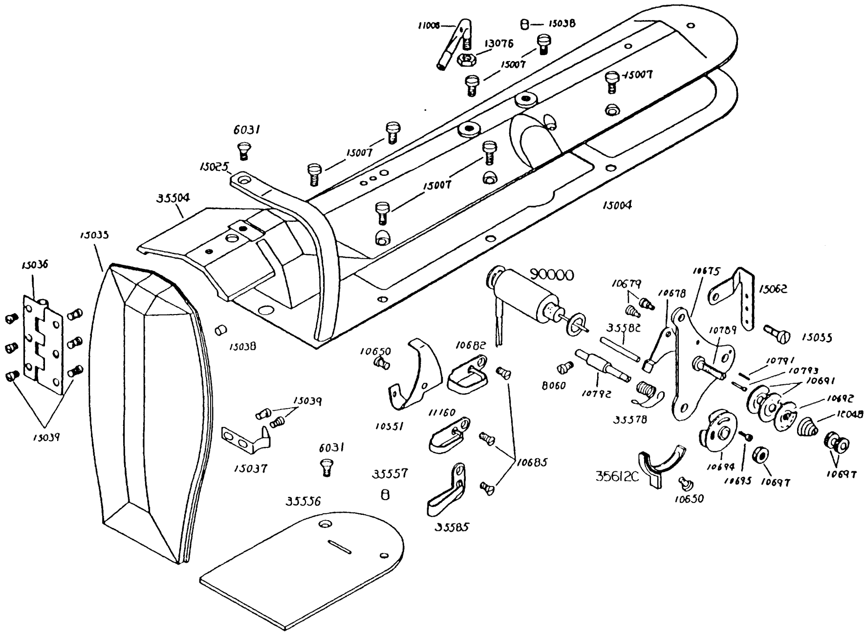
Fig. 7-28: Top Cover, Face Plate, Thread Guide & Thread Tension
